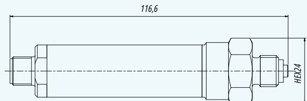
Series 23SX-H2: > 0...120 to 0...1000 bar
