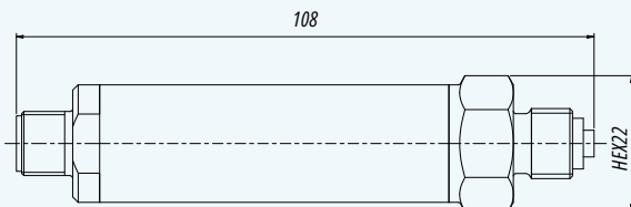
Series 23SX-H2: 0...4 to 0...120 bar
