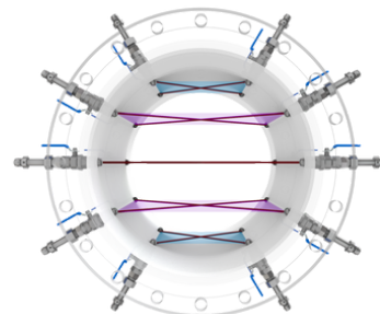
Wetted sensors arranged in five parallel planes
