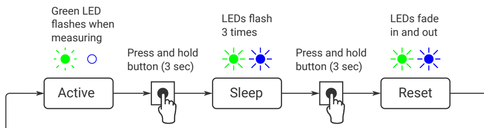
Illustration 1: Switching between active and sleep mode (switch off / on, reset).
