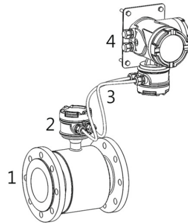
REMOTE VERSION
