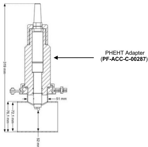
Mounting system for PHEHT sensor (PF-ACC-C-00228)
